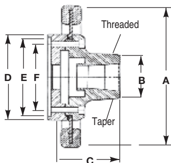
Threaded or taper nose also accepts Hardinge step chucks and closers
