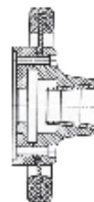
Plain nose for collet applications
