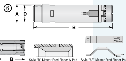
Style "B" Master Feed Finger & Pad
