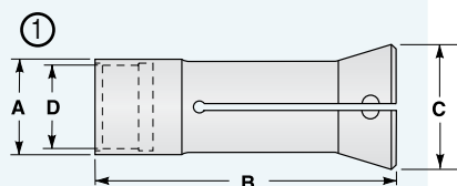
Style "S" Master Collet & Pad
