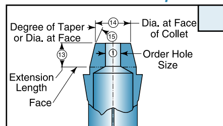
Taper - Reverse
