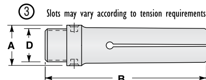
Style "B" Master Feed Finger & Pad
