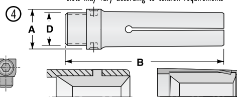
Style "B" Master Feed Finger & Pad
