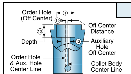
Double-Stepped
