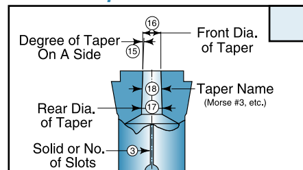
Taper - Reverse
