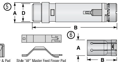
Style "AF" Master Feed Finger Pad
