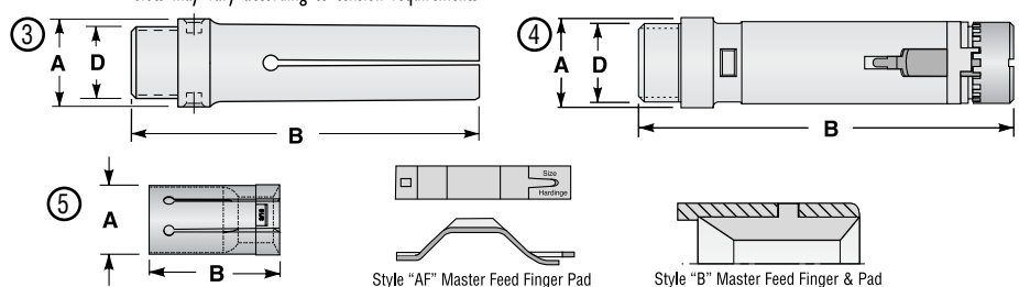
Style "AF" Master Feed Finger Pad
