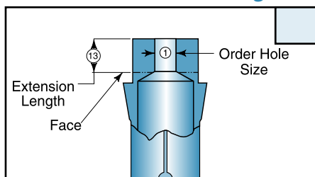
Taper - Regular
