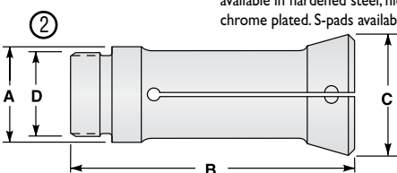
Style "B" Master Feed Finger & Pad
